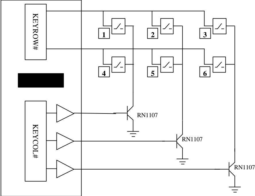
Figure 3.8 Keyboard matrix connections
