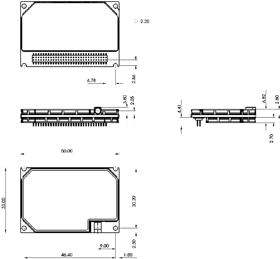
Figure 2.2 Physical dimensions of GR 47/48
