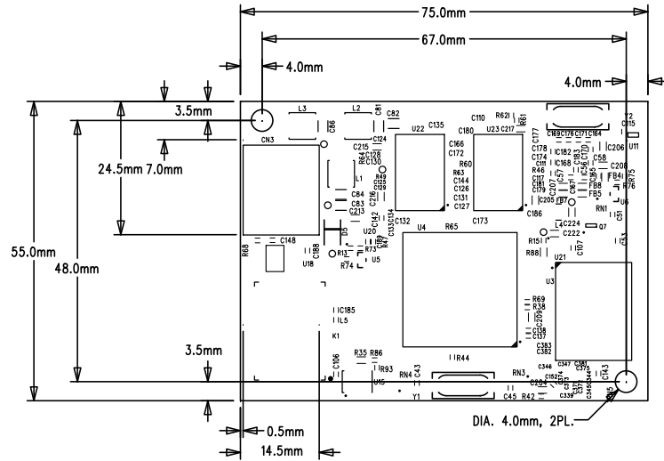
Connector Placement Top View
