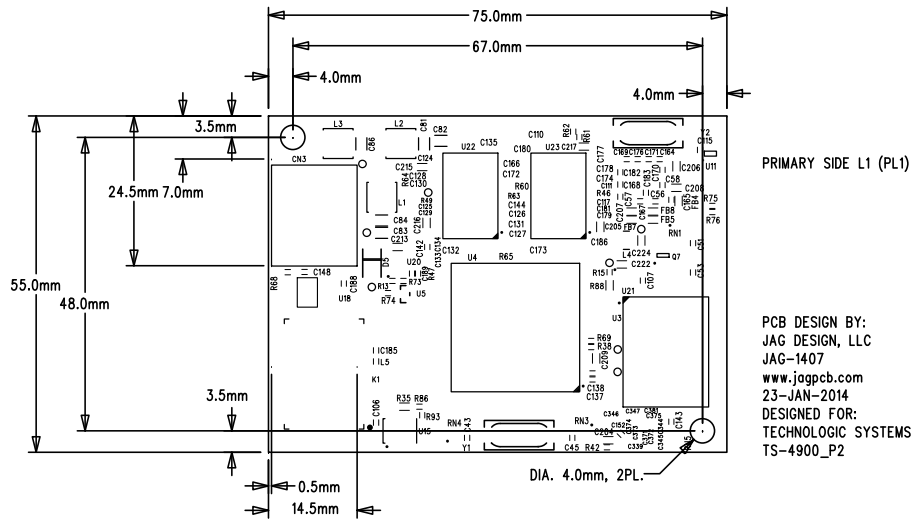
Connector Placement Top View
