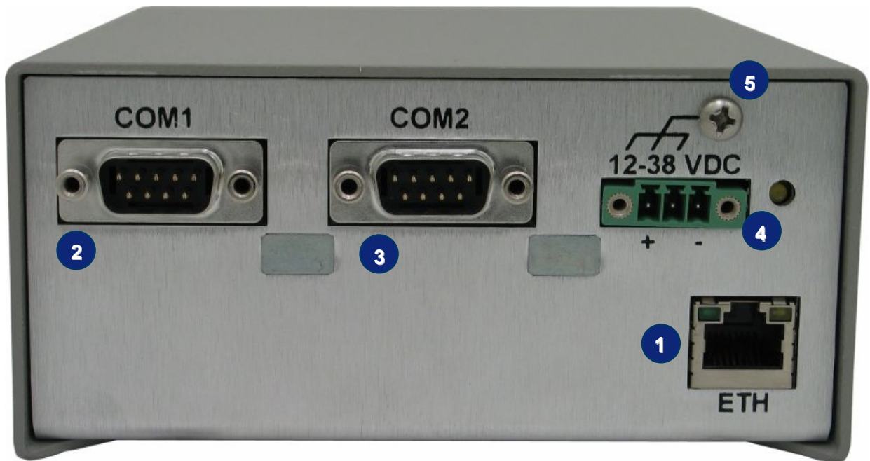
TS Enclosure 560 Rear Panel Connectors
